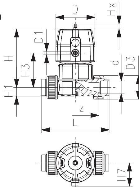
514 Socket/Threaded
